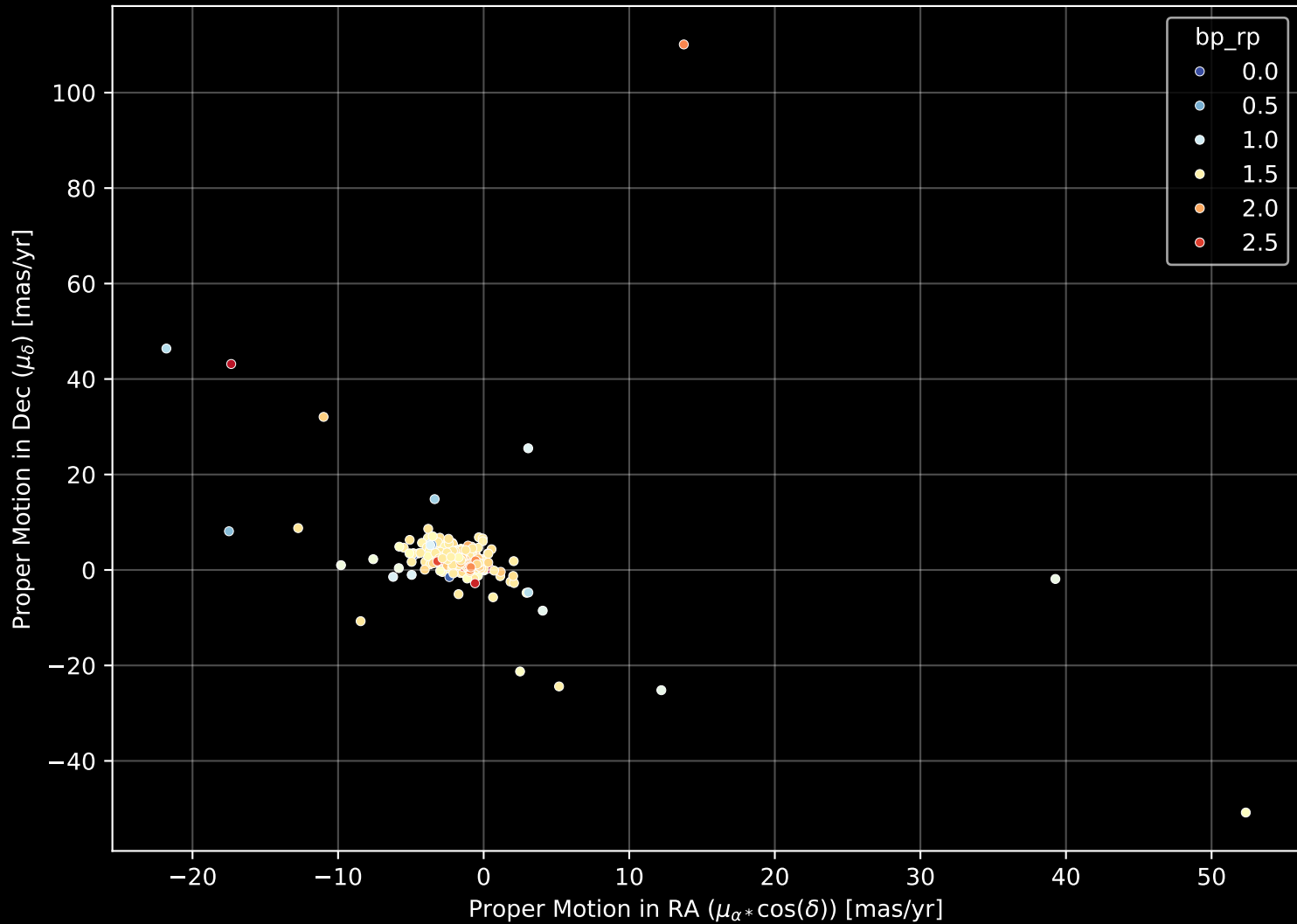
APOGEE DR17 Field: [240+00] Proper Motion Diagram (n= 331)
