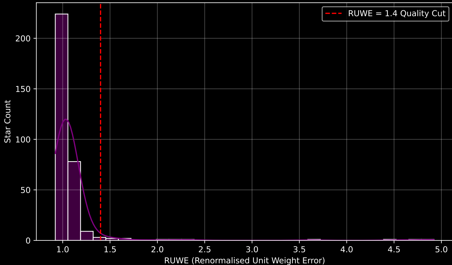
GAPOGEE DR17 Field [240+00] RUWE Distribution (n= 325)
