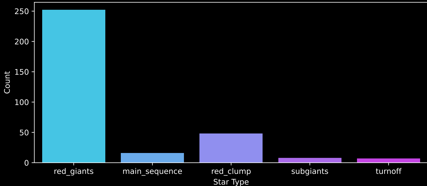
APOGEE DR17 Field: [240+00] Count plot of Star Type
