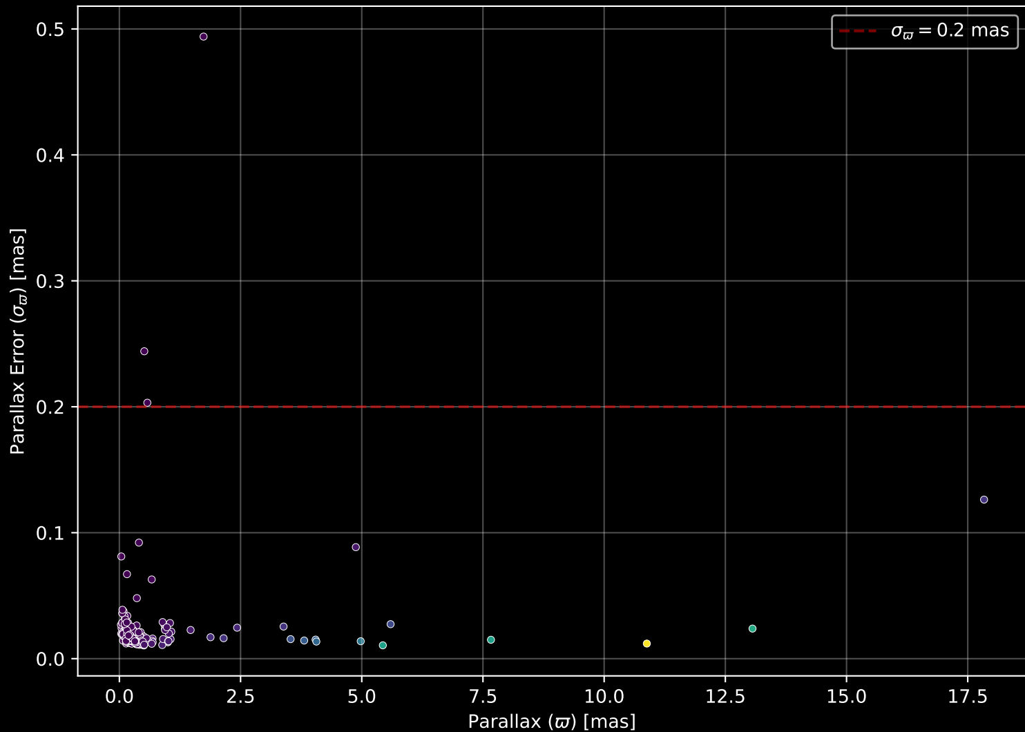
APOGEE DR17 Field: [240+00] Parallax Quality (n= 331)
