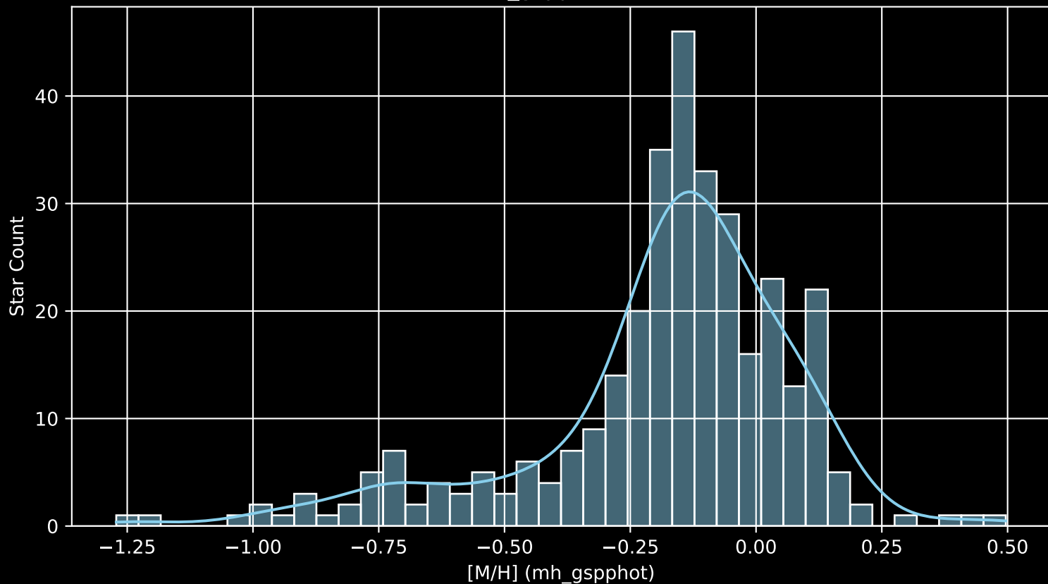
APOGEE DR17 Field: [240+00 [M/H] (mh_gspphot) (n= 329)
